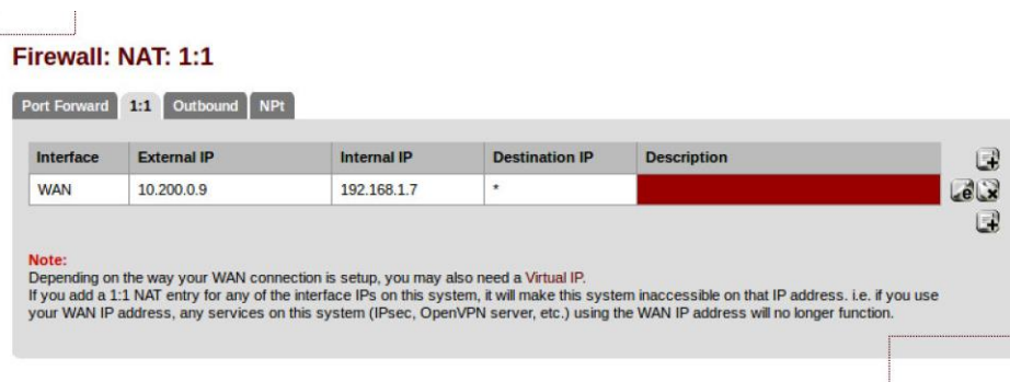
Figure 4: 1:1 NAT settings
