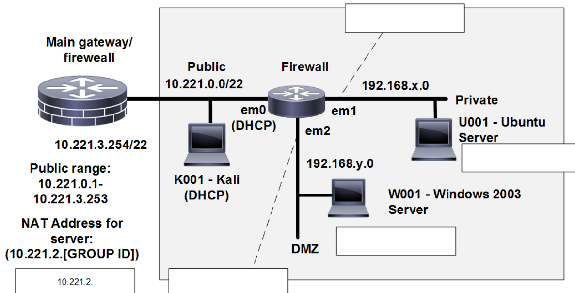
Figure 2: Lab setup
